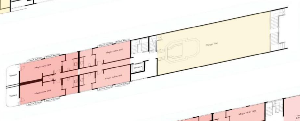
UPPER DECK
